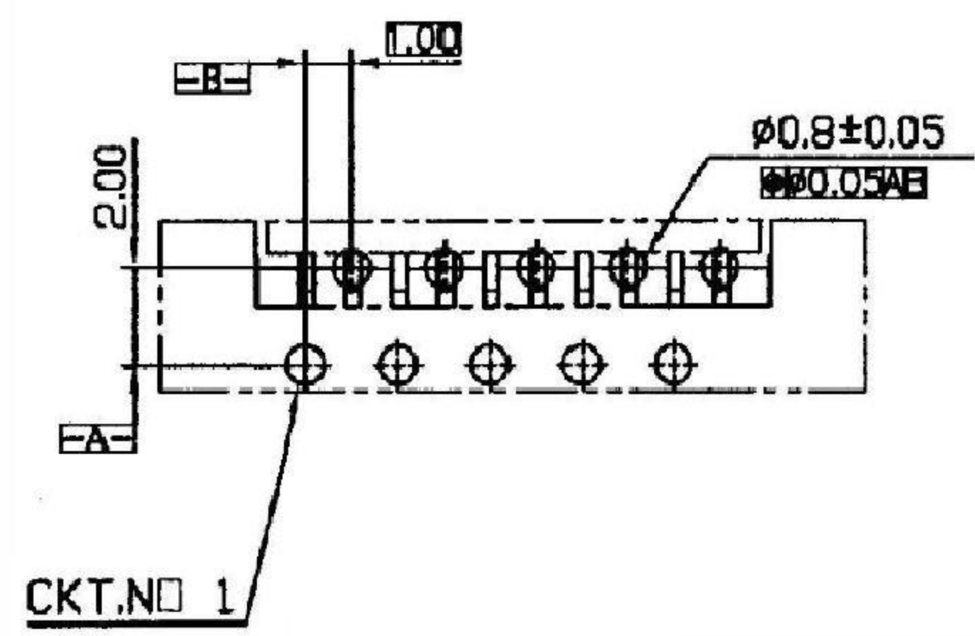
PC BOARD LAYOUT: COMPONENT SIDE
